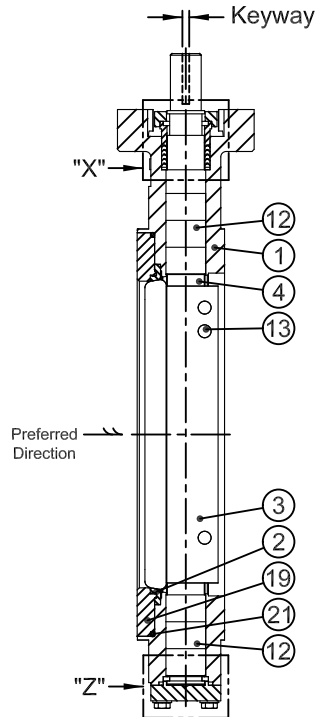
Section View
