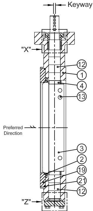
Section View
