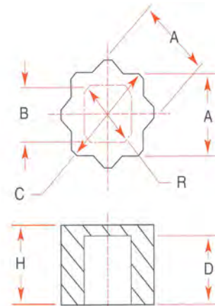
27M14 to 36M27 DESIGN
