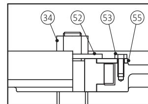
Hammer Blow Handwheel Detail WCB, LCC: NPS 6" & Larger Chrome Alloy: NPS 3" & Larger
