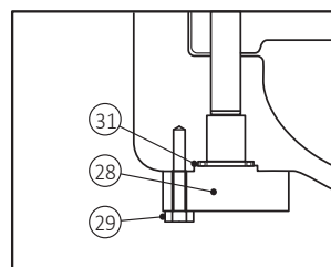
Side Cover Detail Chrome Alloy: NPS 16" Only
