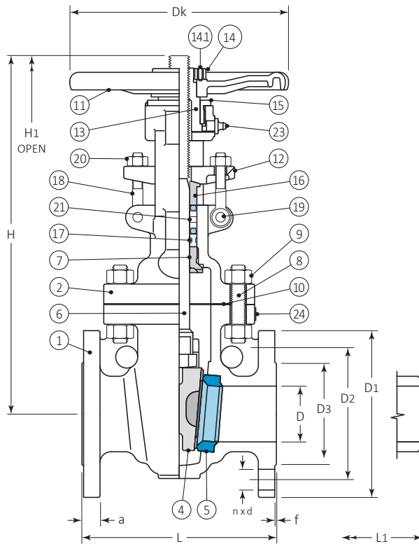
WCB, LCC: NPS 2"-8" Chrome Alloy: NPS 2"-12"
